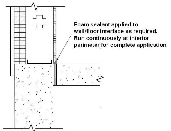
FIGURE 3—WALL FLOOR JUNCTURE
